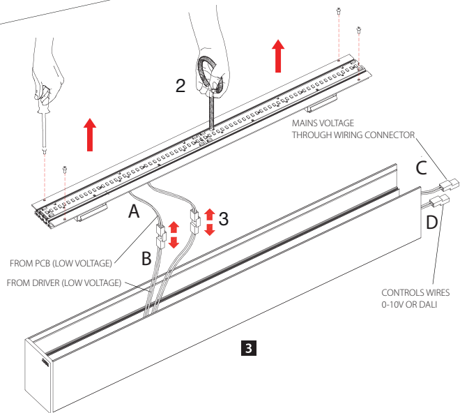
2- THREADED HANDLE FOR HANDLING COMPONENT TRAY
