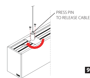
8 HOLD THE LUMINAIRE WHILE PRESSING THE PIN
